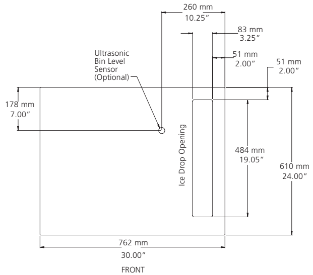
30" Prodigy plan view
